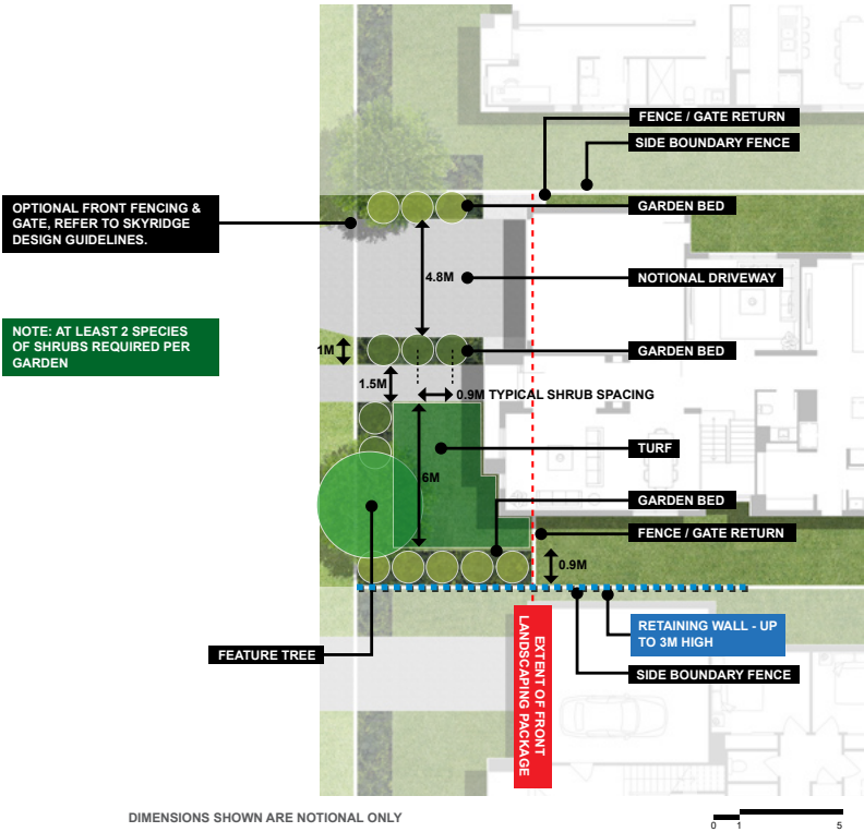
PLAN VIEW
